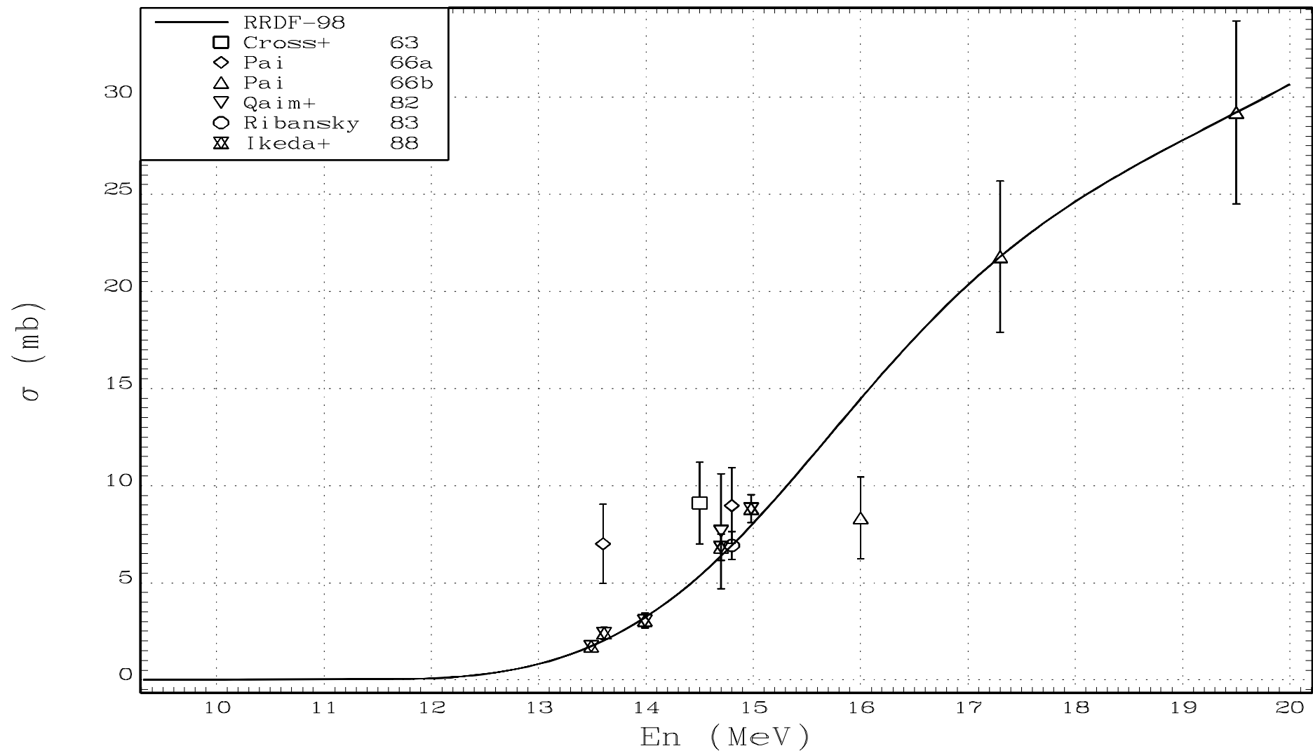
Fig.10. RRDF-98 evaluated excitation function for the ^{49}\text{Ti}(n,x)^{48}\text{Sc} reaction in comparison with the experimental data.
