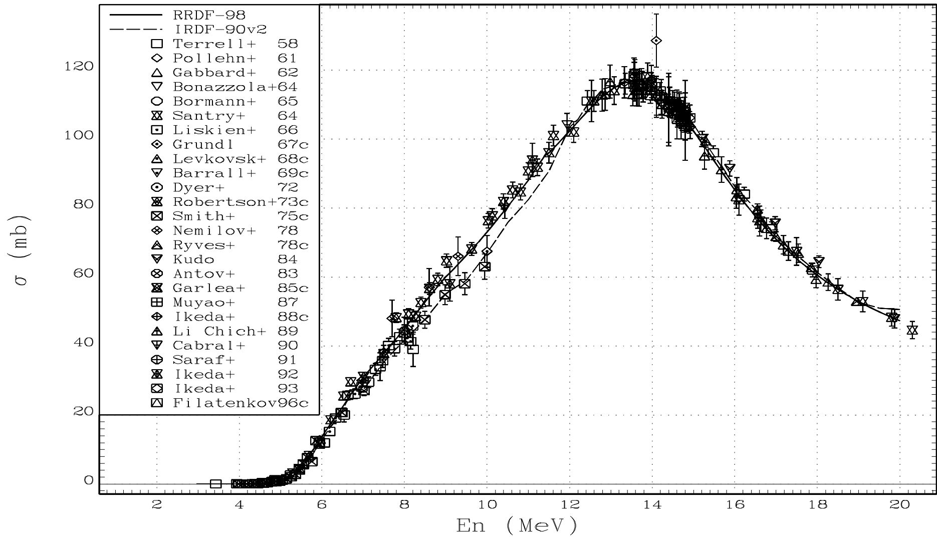
Fig.14. RRDF-98 evaluated excitation function for the ^{56}\text{Fe}(n,p)^{56}\text{Mn} reaction in comparison with IRDF-90 (version 2) curve and experimental data.
