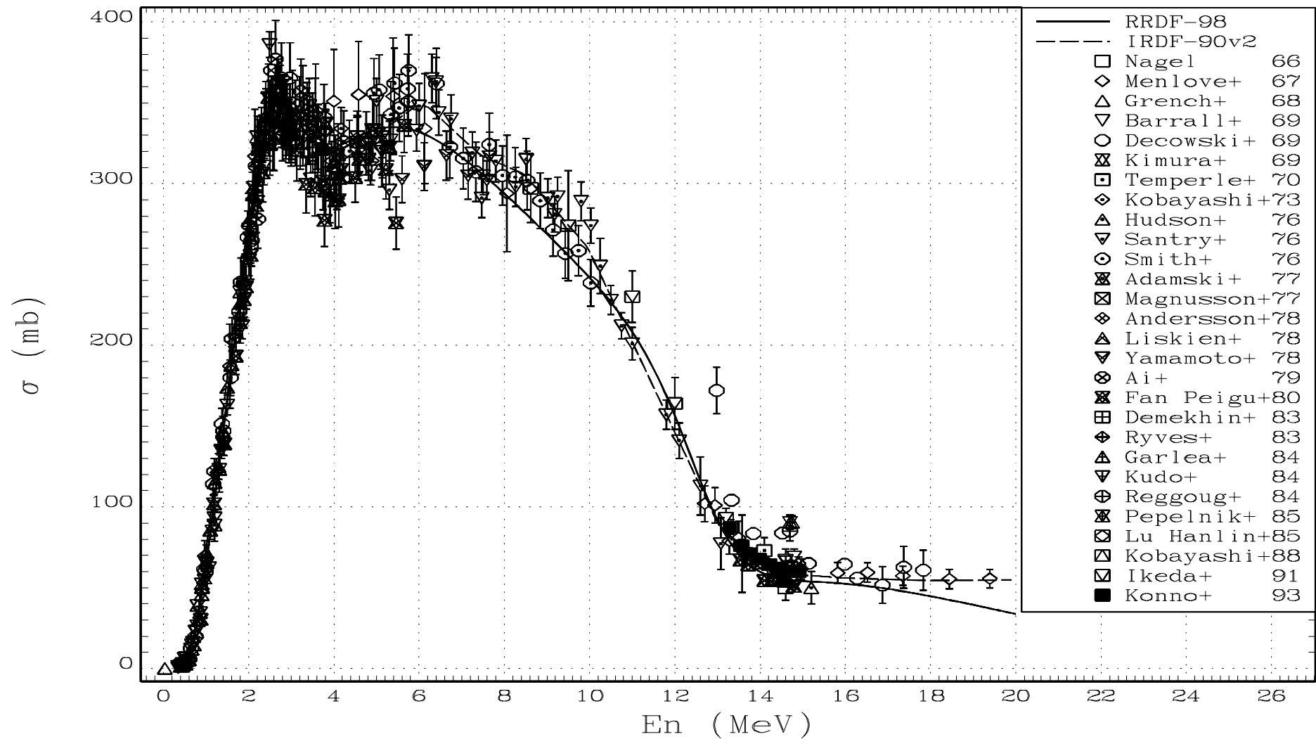
Fig.21. RRDF-98 evaluated excitation function for the ^{115}\text{In}(n,n')^{115\text{m}}\text{In} reaction in comparison with IRDF-90 (version 2) curve and experimental data.
