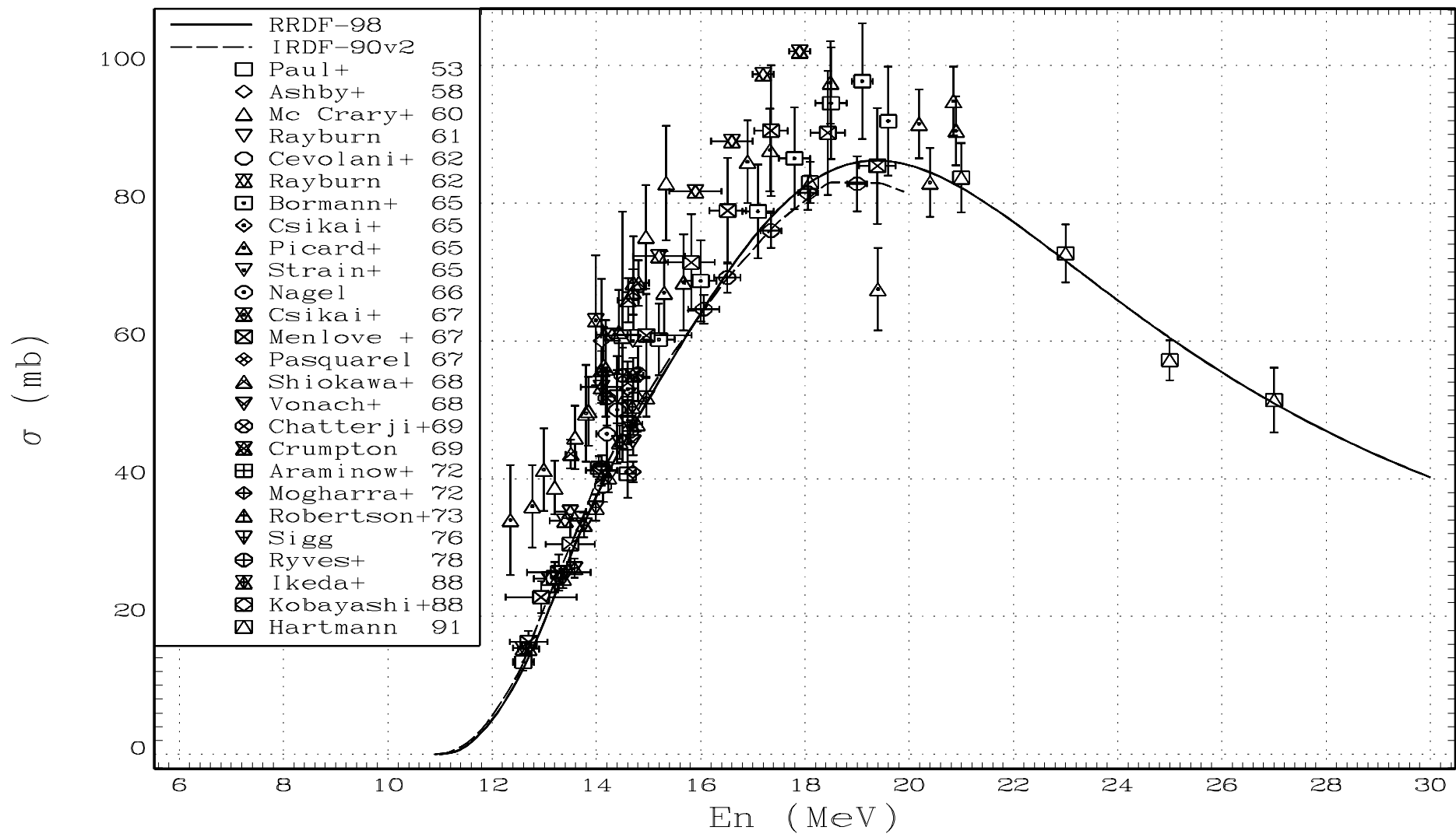
Fig.3. RRDF-98 evaluated excitation function for the ^{19}\text{F}(n,2n)^{18}\text{F} reaction in comparison with IRDF-90 (version 2) curve and experimental data.
