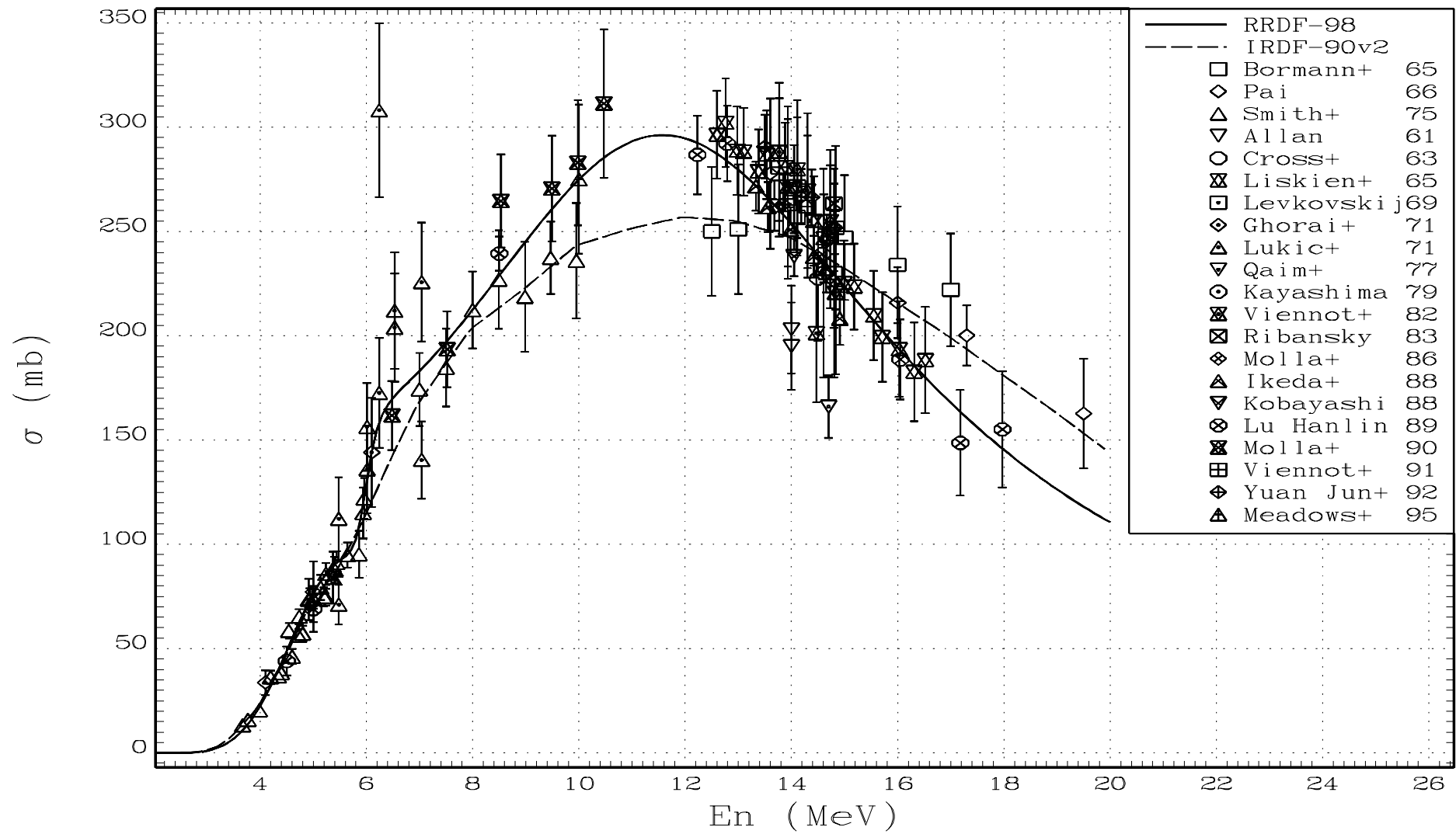
Fig.6. RRDF-98 evaluated excitation function for the ^{46}\text{Ti}(n,p)^{46}\text{Sc} reaction in comparison with IRDF-90 (version 2) curve and experimental data.
