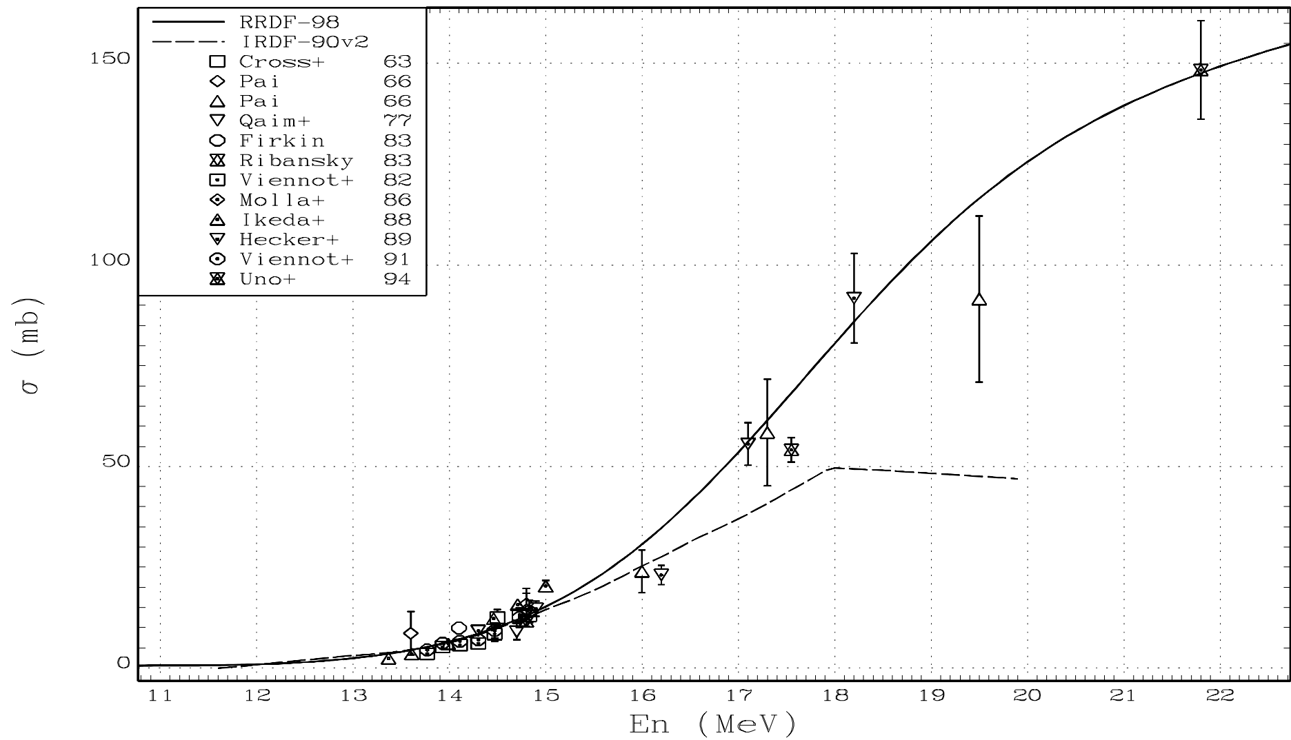
Fig.8. RRDF-98 evaluated excitation function for the ^{48}\text{Ti}(n,x)^{47}\text{Sc} reaction in comparison with IRDF-90 (version 2) curve and experimental data.
